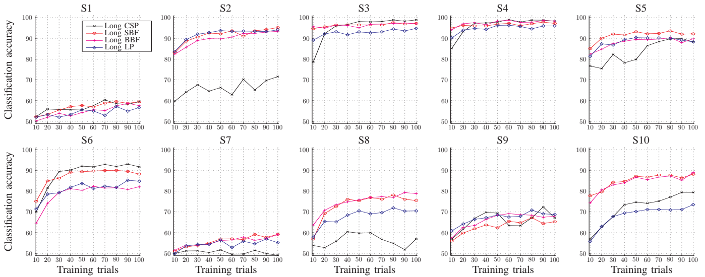
Fig. 1. Classification accuracies in percent for subjects S1-S10 using the long time window as a function of the number of training trials per condition for spatial filtering by Common Spatial Patterns (CSP), static Beamforming (SBF), block-adaptive Beamforming (BBF), and Laplacian spatial filtering (LP).
