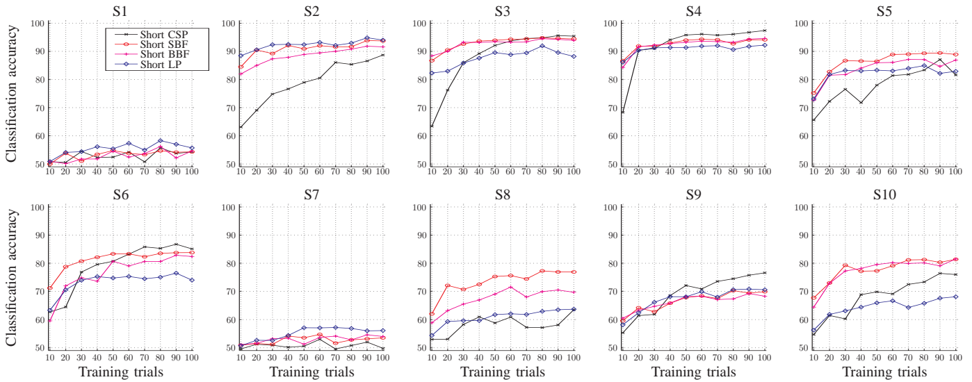
Fig. 2. Classification accuracies in percent for subjects S1-S10 using the short time window as a function of the number of training trials per condition for spatial filtering by Common Spatial Patterns (CSP), static Beamforming (SBF), block-adaptive Beamforming (BBF), and Laplacian spatial filtering (LP).
