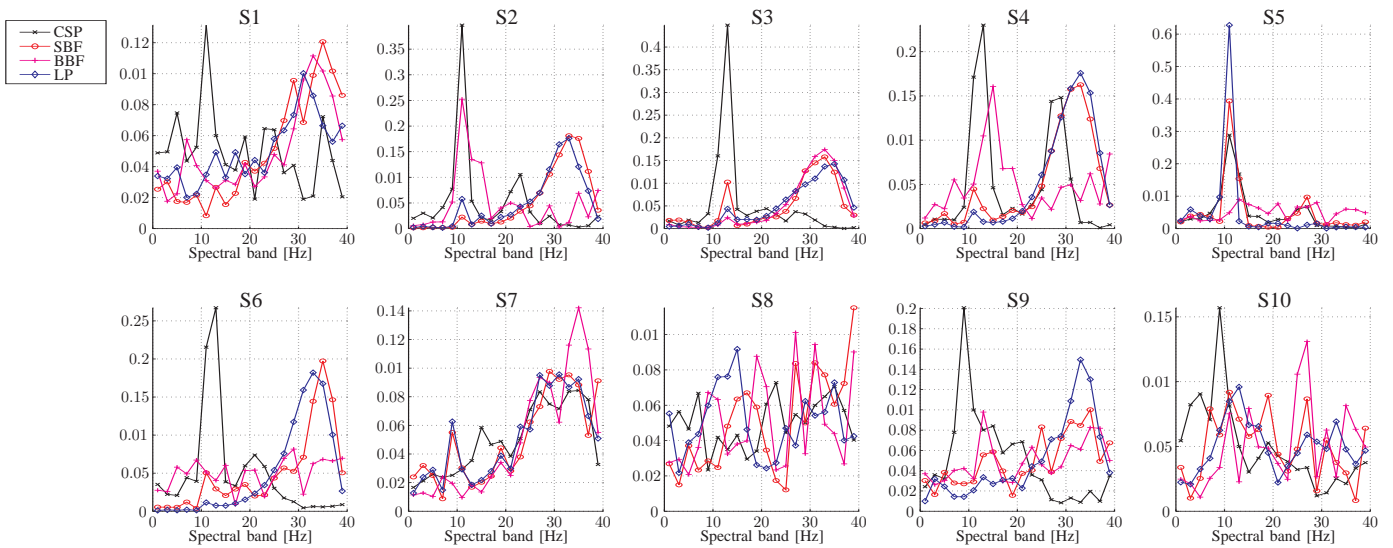
Fig. 3. Normalized mean absolute weights of different spectral bands across all training set sizes and both time windows as determined by the l_1 -regularized logistic regression classifier for Common Spatial Patterns (CSP), static Beamforming (SBF), block-adaptive Beamforming (BBF), and Laplacian spatial filtering (LP).
